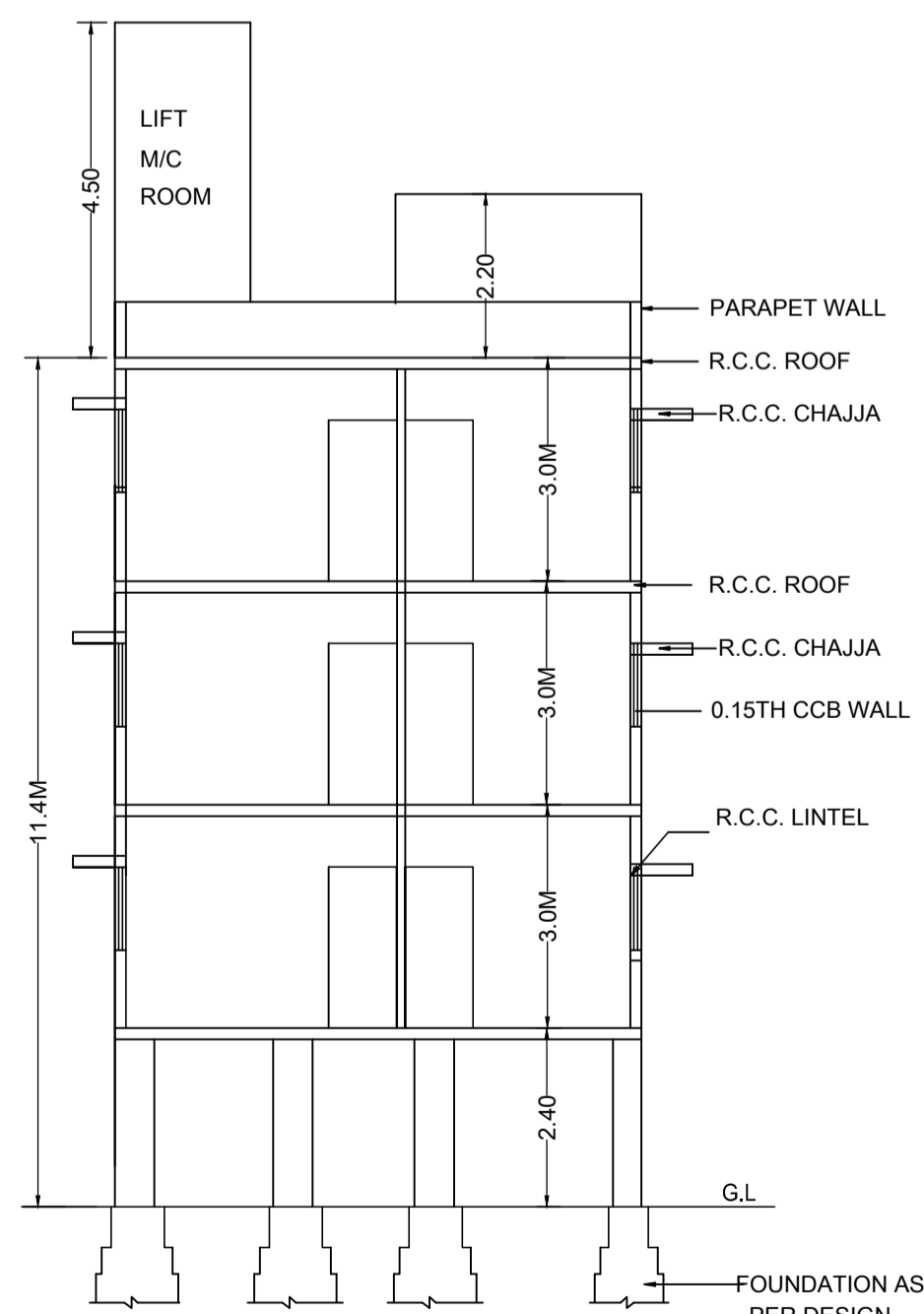
SECTION AT 'AA'
